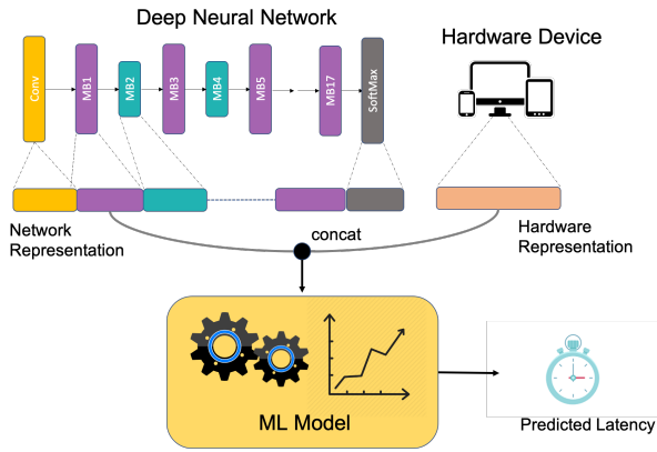
Fig. 7. This diagram shows our proposed cost model that takes in the representation of DNN and hardware as input to predict the latency of that DNN on that hardware. We represent each DNN by recursively encoding the layer identifier (one-hot) and its parameters. Each hardware is represented using a vector containing measured inference latencies on the signature set. We use XGBoost to train our cost model on inference latency data.
